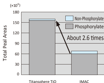
Comparison of Phosphorylated Peptide Recovery Amount
